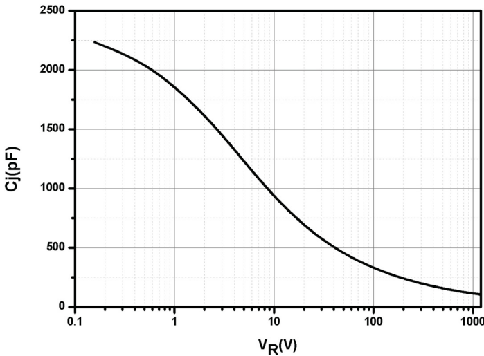
FIGURE 3. Capacitance Versus Reverse Voltage
