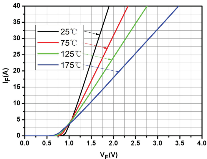
FIGURE 1. Forward Voltage Characteristics
