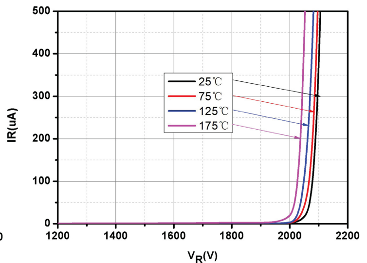
FIGURE 2. Reverse Characteristics
