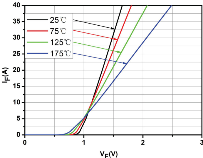
FIGURE 1. Forward Voltage Characteristics
