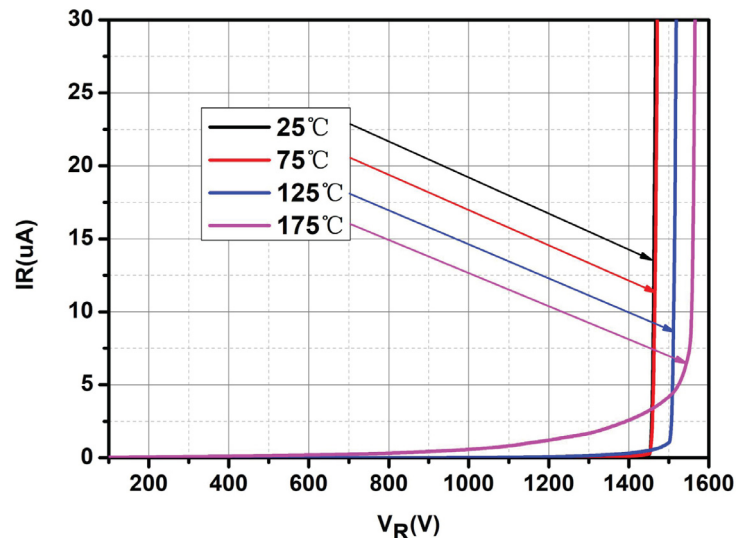
FIGURE 2. Reverse Characteristics
