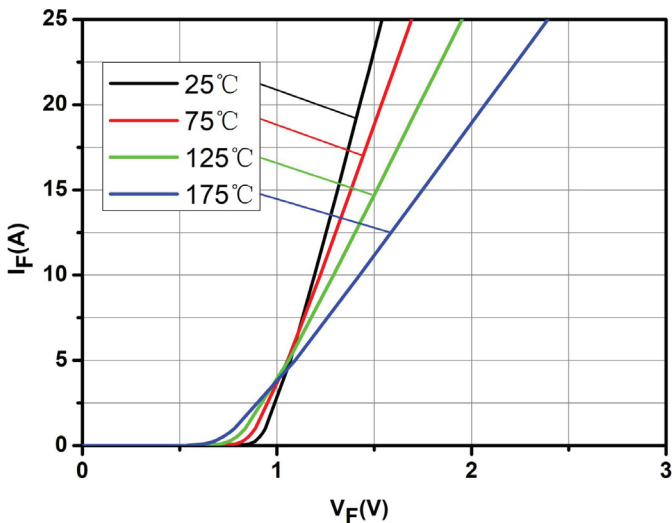
FIGURE 1. Forward Voltage Characteristics
