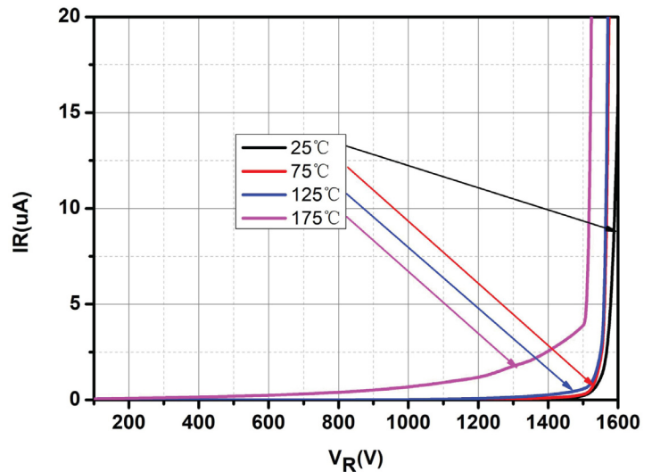
FIGURE 2. Reverse Characteristics
