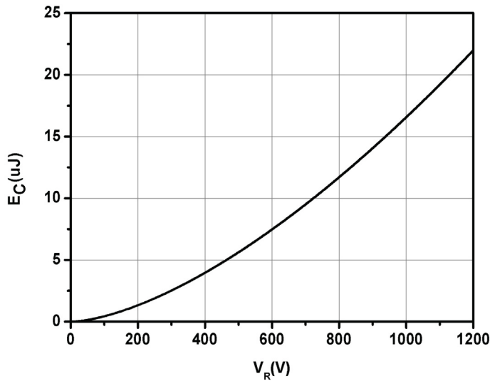
FIGURE 5. Capacitance Stored Energy
