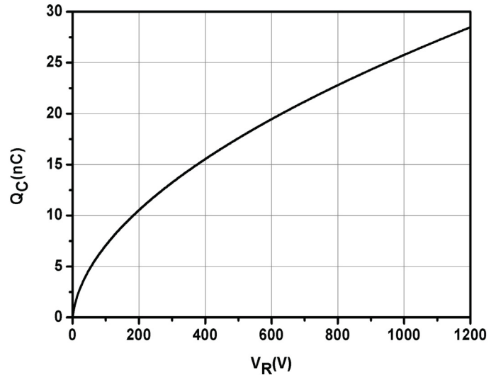
FIGURE 4. Total Capacitance Charge Versus Reverse Voltage
