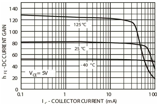
Fig 1 - Typical Pulsed Current Gain versus Collector Current
