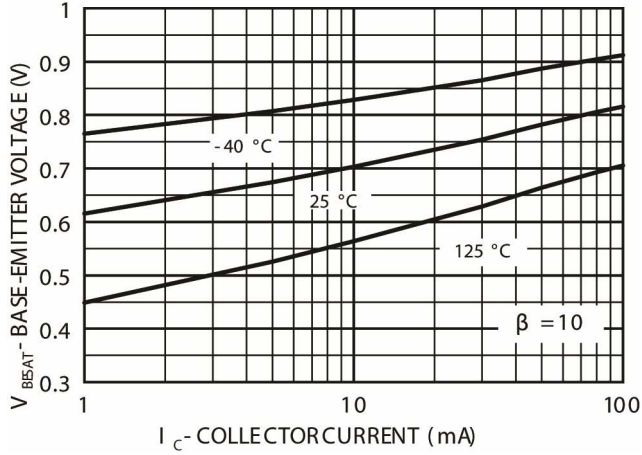
Fig 3 - Base-Emitter Saturation Voltage versus Collector Current
