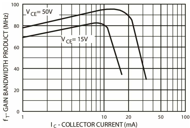
Fig 5 - Gain Bandwidth Product versus Collector Current
