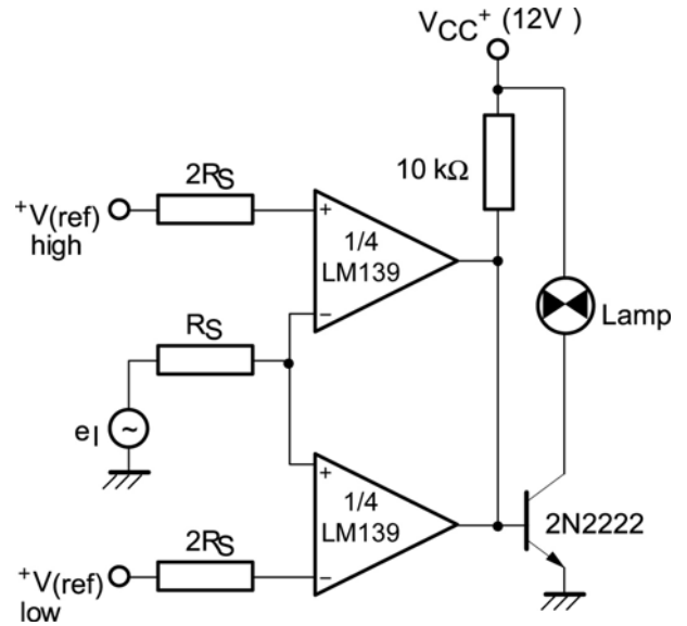
FIGURE 14. Limit Comparator
