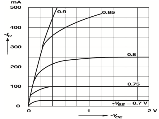
Fig 8 – Common Emitter Collector characteristics
