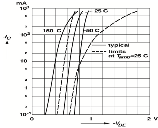
Fig 1 – Collector Current versus Base-Emitter Voltage
