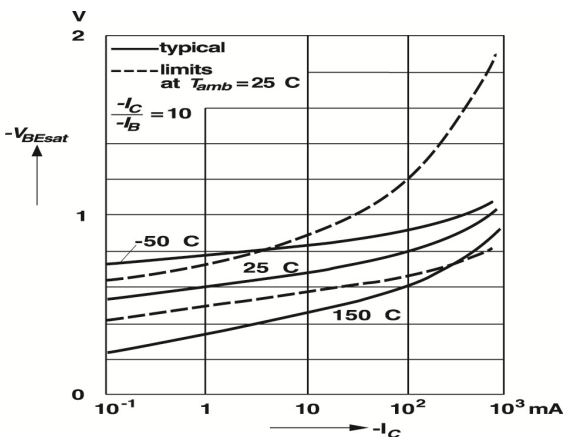
Fig 5 – Base Saturation Voltage versus Collector Current
