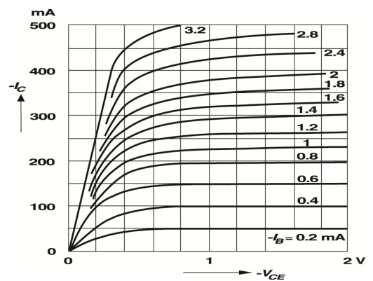
Fig 6 – Common Emitter Collector characteristics
