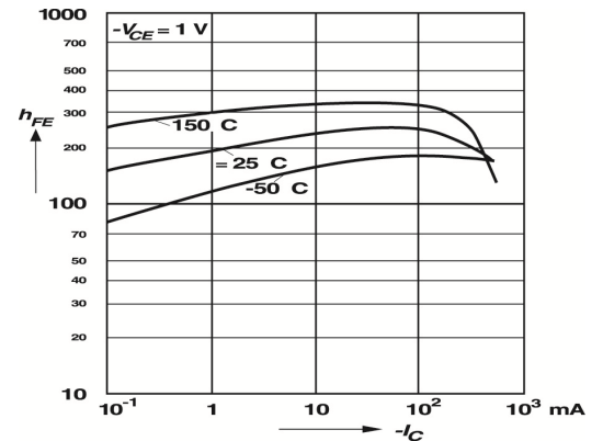
Fig 4 – Current Gain versus Collector Current
