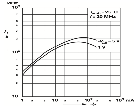
Fig 2 – Gain-bandwidth product versus Collector Current
