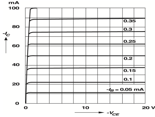
Fig 7 – Common Emitter Collector characteristics
