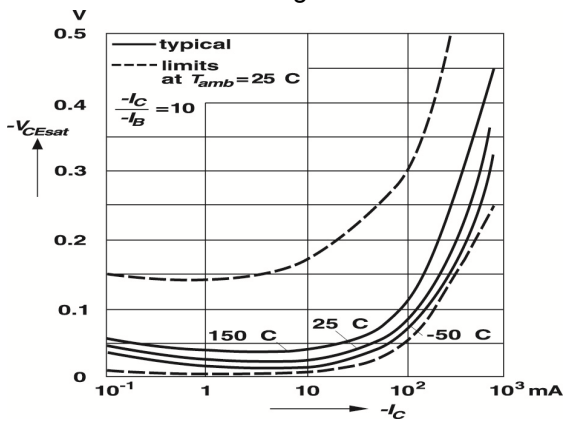
Fig 3 – Collector Saturation Voltage versus Collector Current
