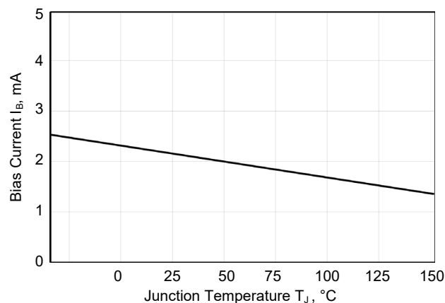
Figure 1 – Bias Current Versus Temperature
