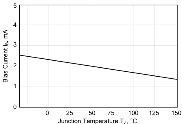
Figure 3 – Bias Current Versus Temperature
