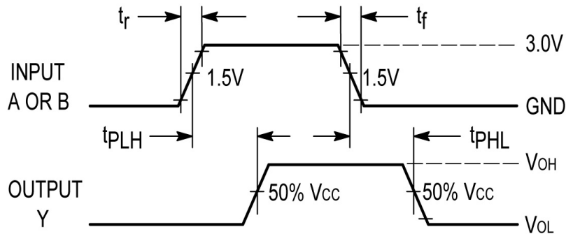
Figure 1 – Propagation Delay
