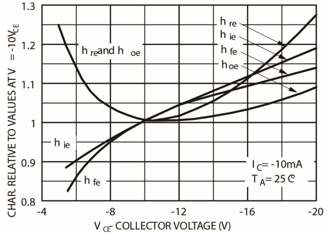
Fig 11 – Common Emitter Characteristics
