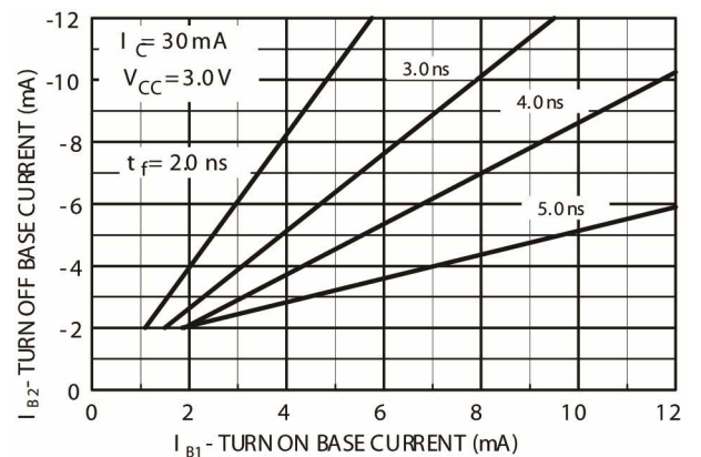
Fig 11 - Fall Time versus Turn On and Turn Off Base Currents
