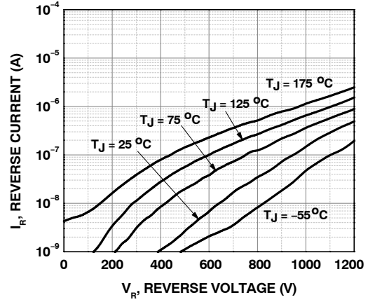
Figure 5. Reverse Characteristics
