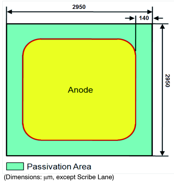
Figure 1. Die Layout
