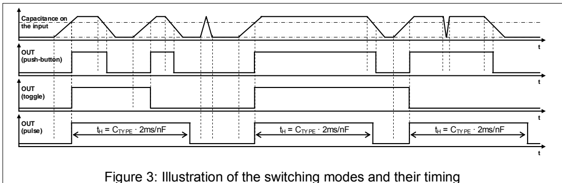
Figure 3 illustrates the switching behaviour for the three modes. Additionally the graph illustrates, that short term disturbances on the sensor are suppressed by the circuit.
