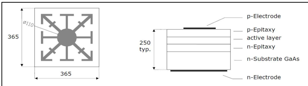
Chip thickness: typ. 250 µm, electrodes / metallization - Au alloy
