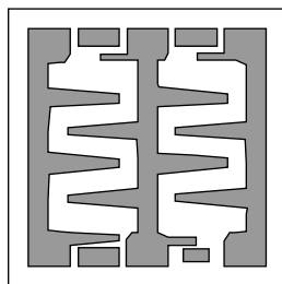
TYPICAL RANGE 10 \Omega to 26.9 \Omega
