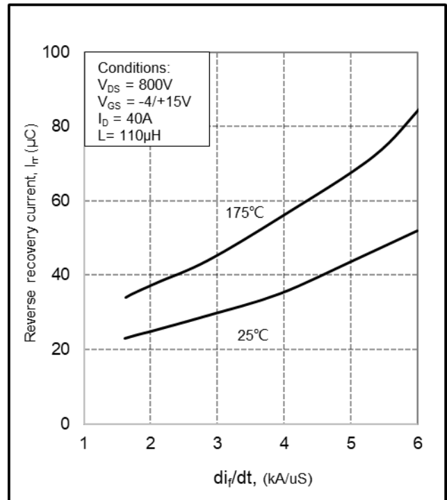
Figure 20. Reverse recovery current vs. di_f/dt
