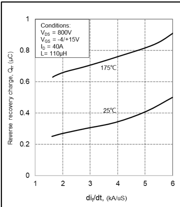
Figure 19. Reverse recovery charge vs. di_f/dt
