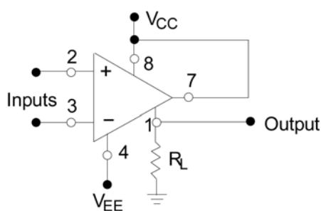
Ground Referred Load (Input polarity reversed if GND is output)
