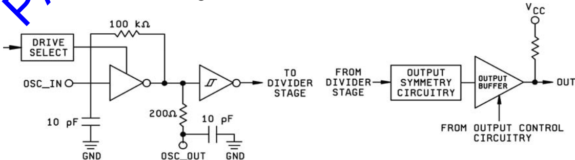
Output Stage
