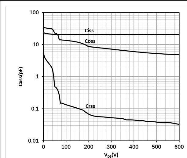
Figure 19 Typ. capacitances
