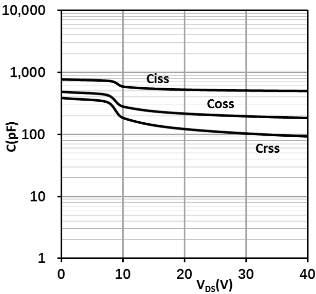
Fig. 11 Typ. Capacitances Characteristics
