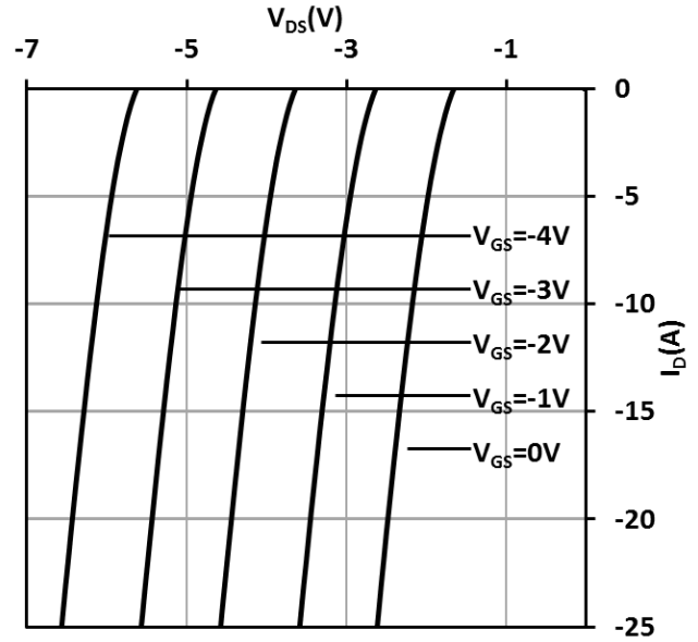
Fig. 10 Typ. Reverse Drain-Source Characteristics
