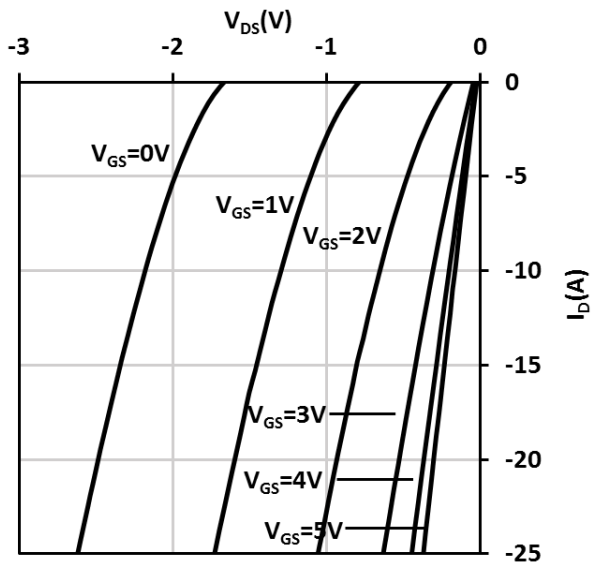
Fig. 9 Typ. Reverse Drain-Source Characteristics
