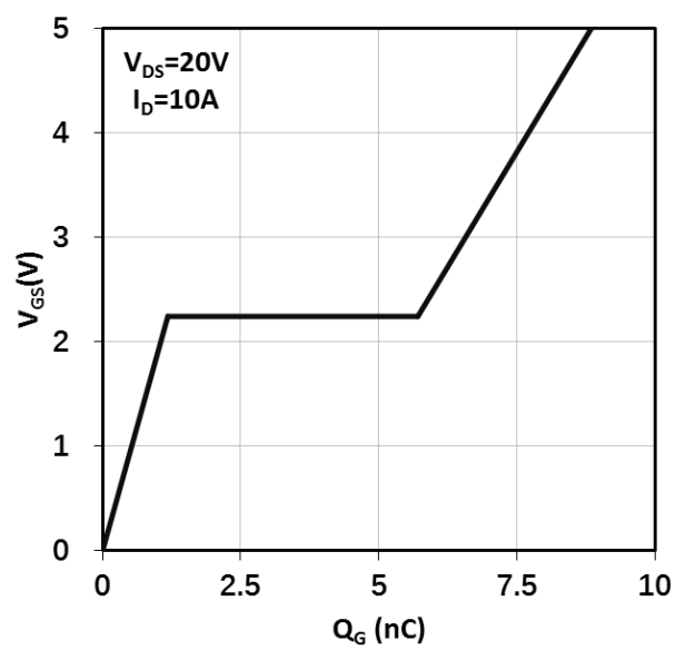
Fig. 12 Typ. Gate Charge
