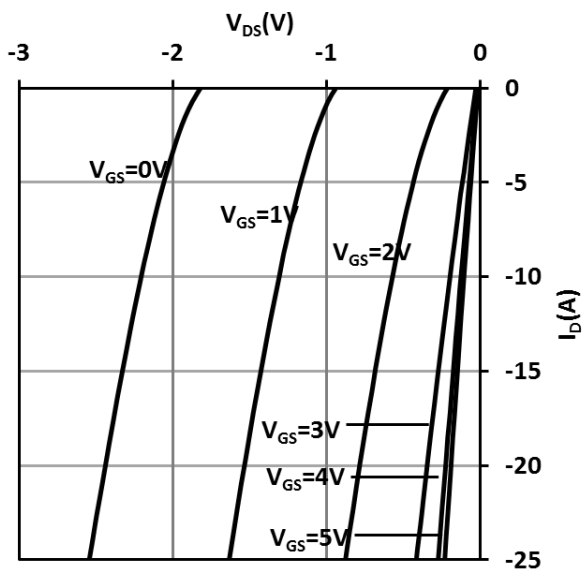
Fig. 7 Typ. Reverse Drain-Source Characteristics
