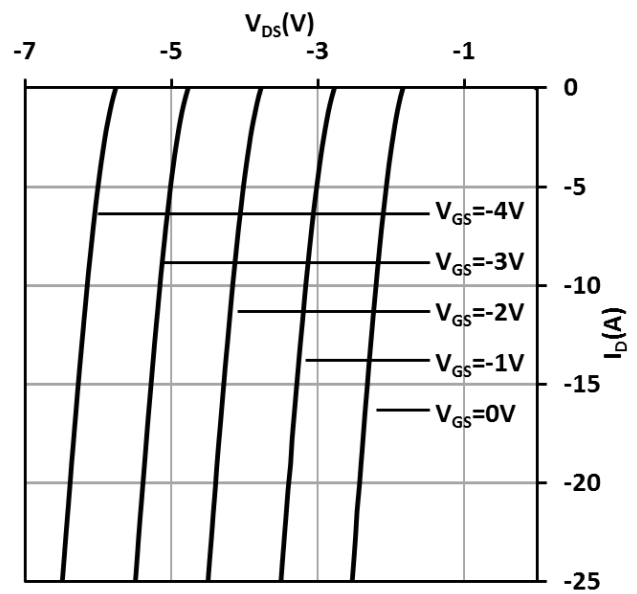
Fig. 8 Typ. Reverse Drain-Source Characteristics
