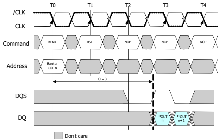
Figure 18 : Read Burst terminate (BL=4 or 8)
