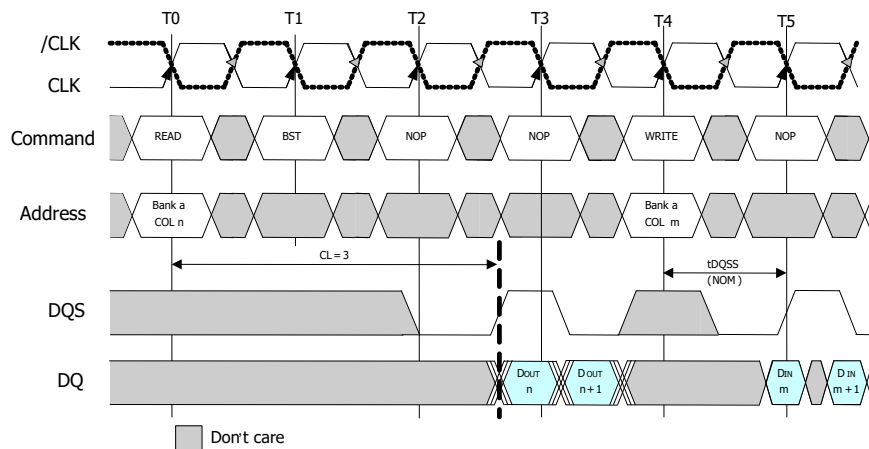
Figure 19 : Read to write terminate (BL=4 or 8)
