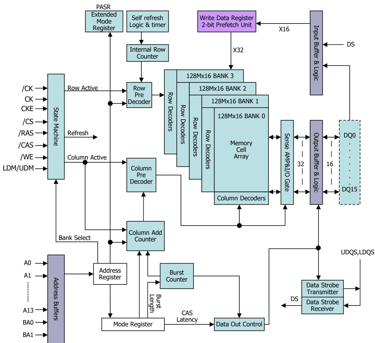
Figure 2.1 : Functional Block Diagram (128Mb X 16)
