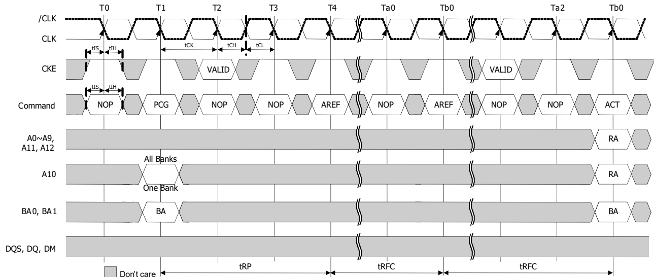
Figure 34 : Auto refresh
