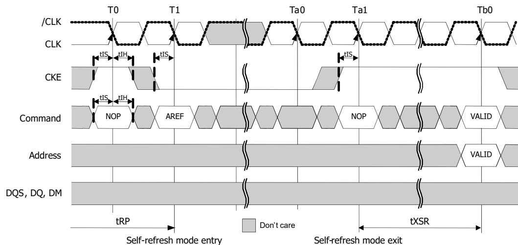
Figure 35 : Self refresh
