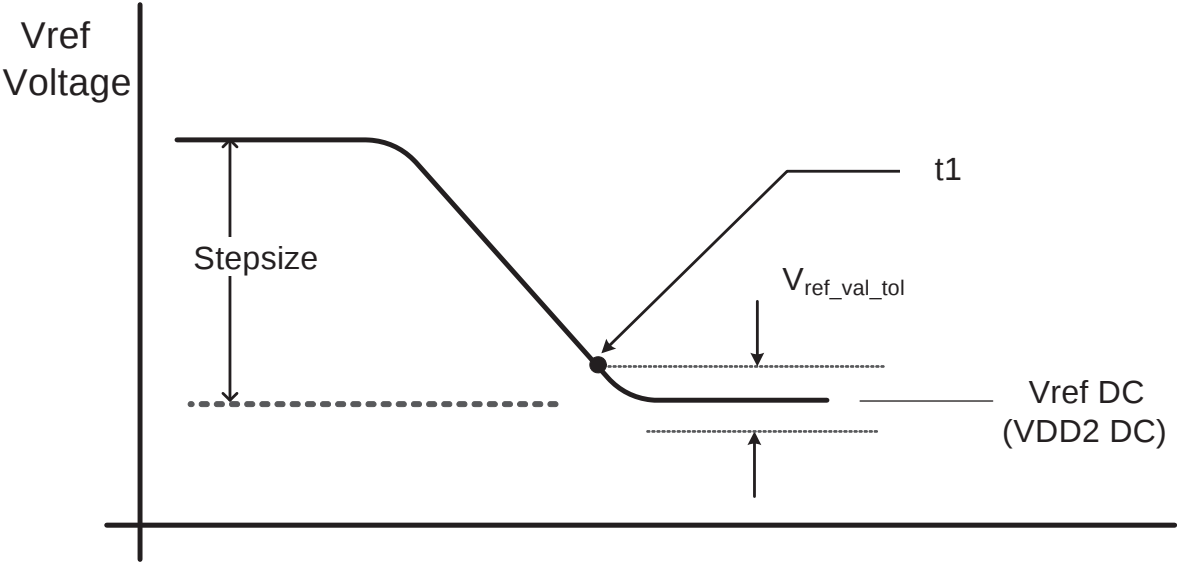
4.73 — V_{REF} step single stepsize decrement case
