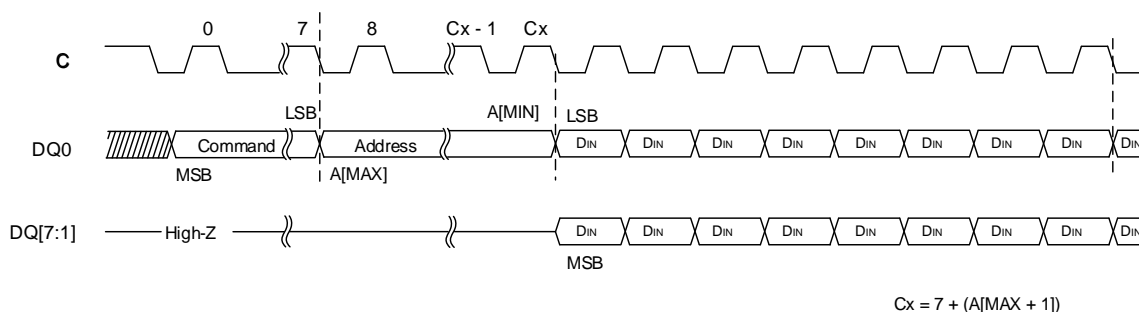
Figure 8.17 OCTAL INPUT FAST PROGRAM – 82h/84h
