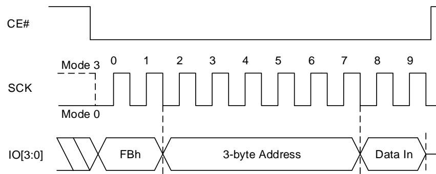
Figure 8.117 Write DYB Sequence In QPI Mode (FBh [EXTADD=0], 3-byte address)
