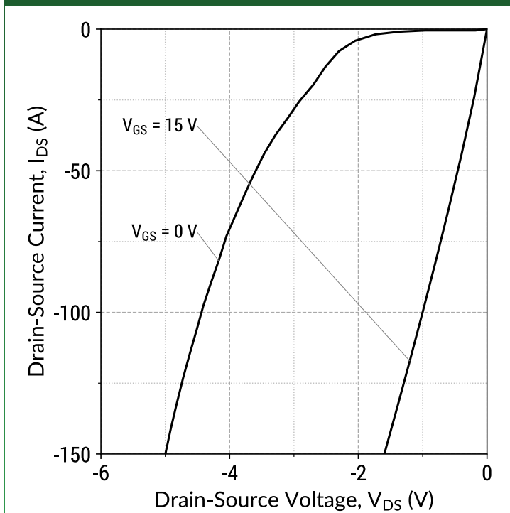
Figure 15: Third Quadrant Characteristics ( T_j = 25^\circ\text{C} )
