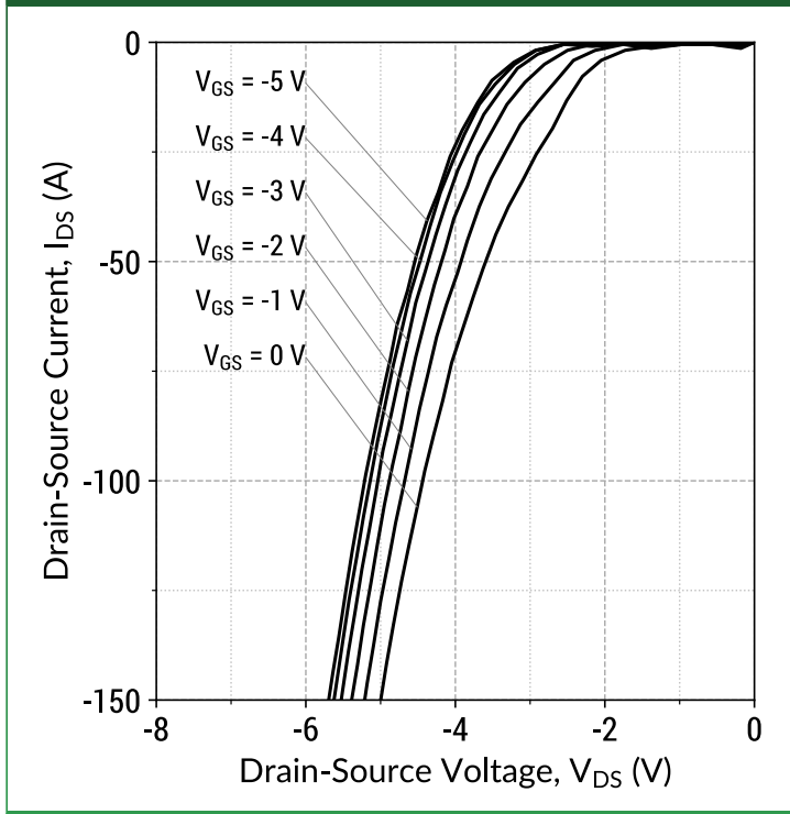
Figure 13: Body Diode Characteristics ( T_j = 25^\circ\text{C} )
