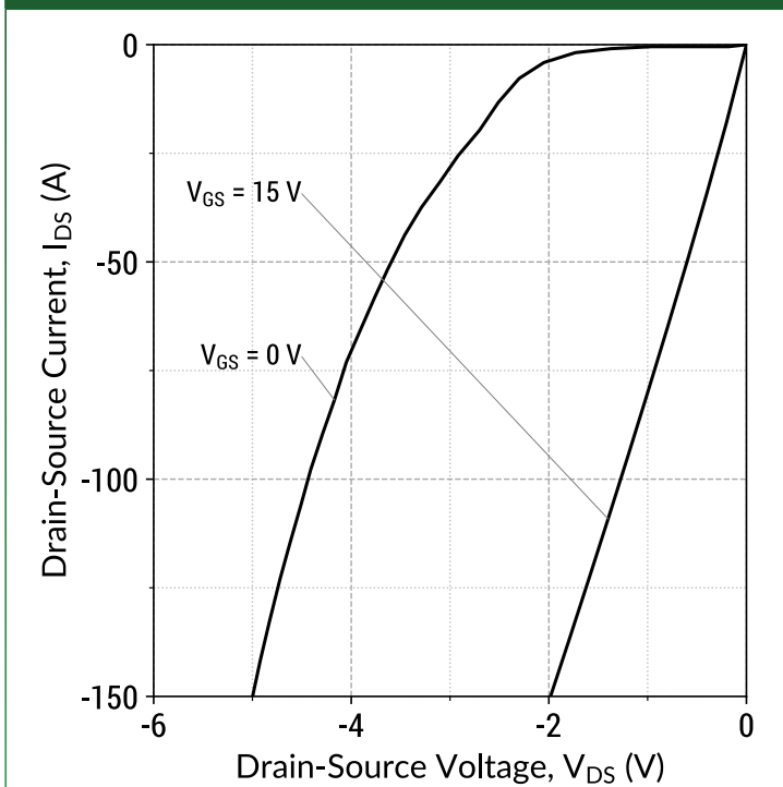
Figure 16: Third Quadrant Characteristics ( T_j = 200^\circ\text{C} )
